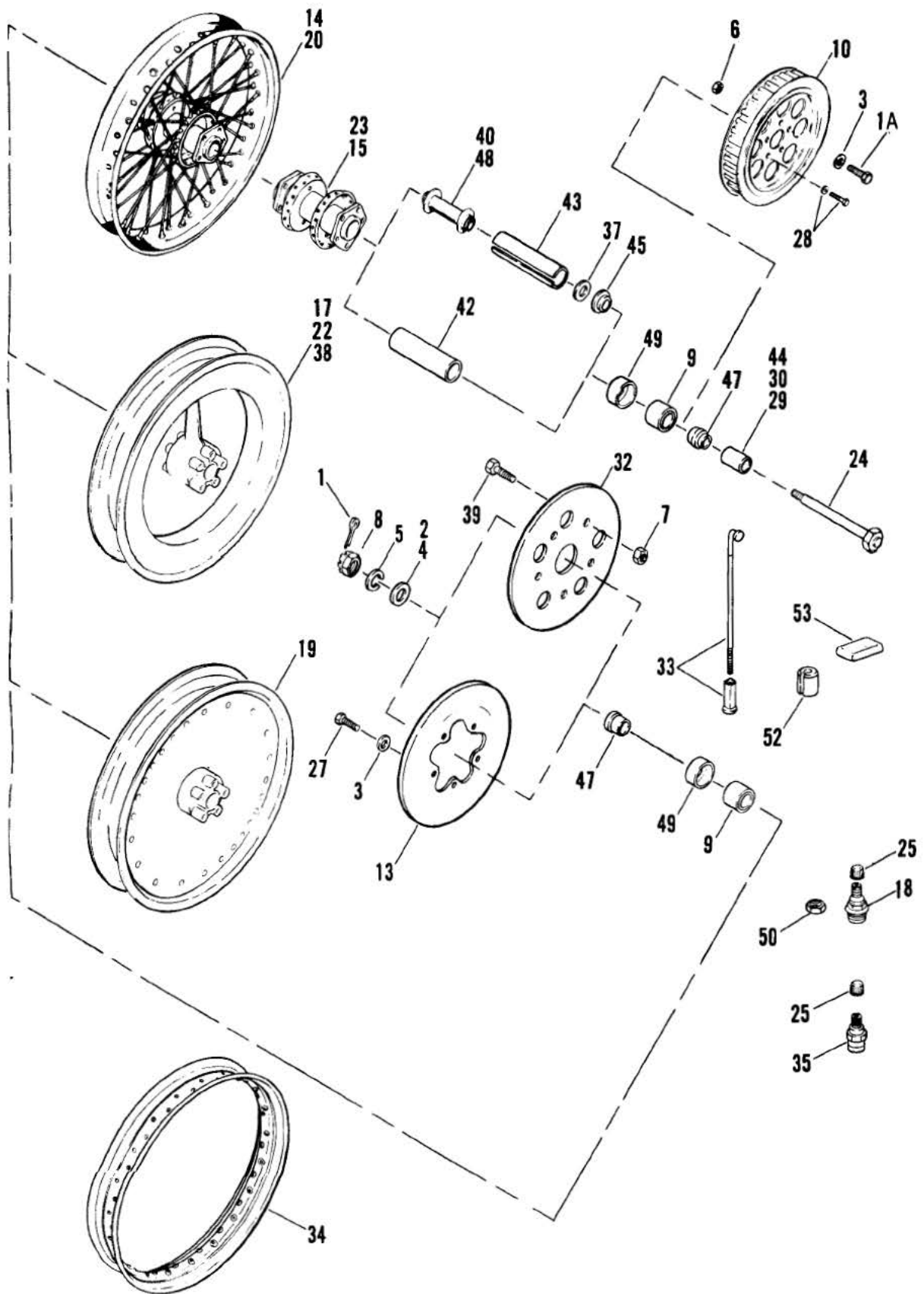
REAR WHEEL
