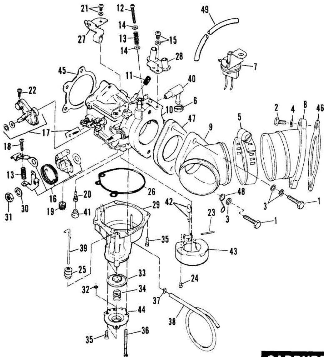
CARBURETOR 1987 TO 1989
