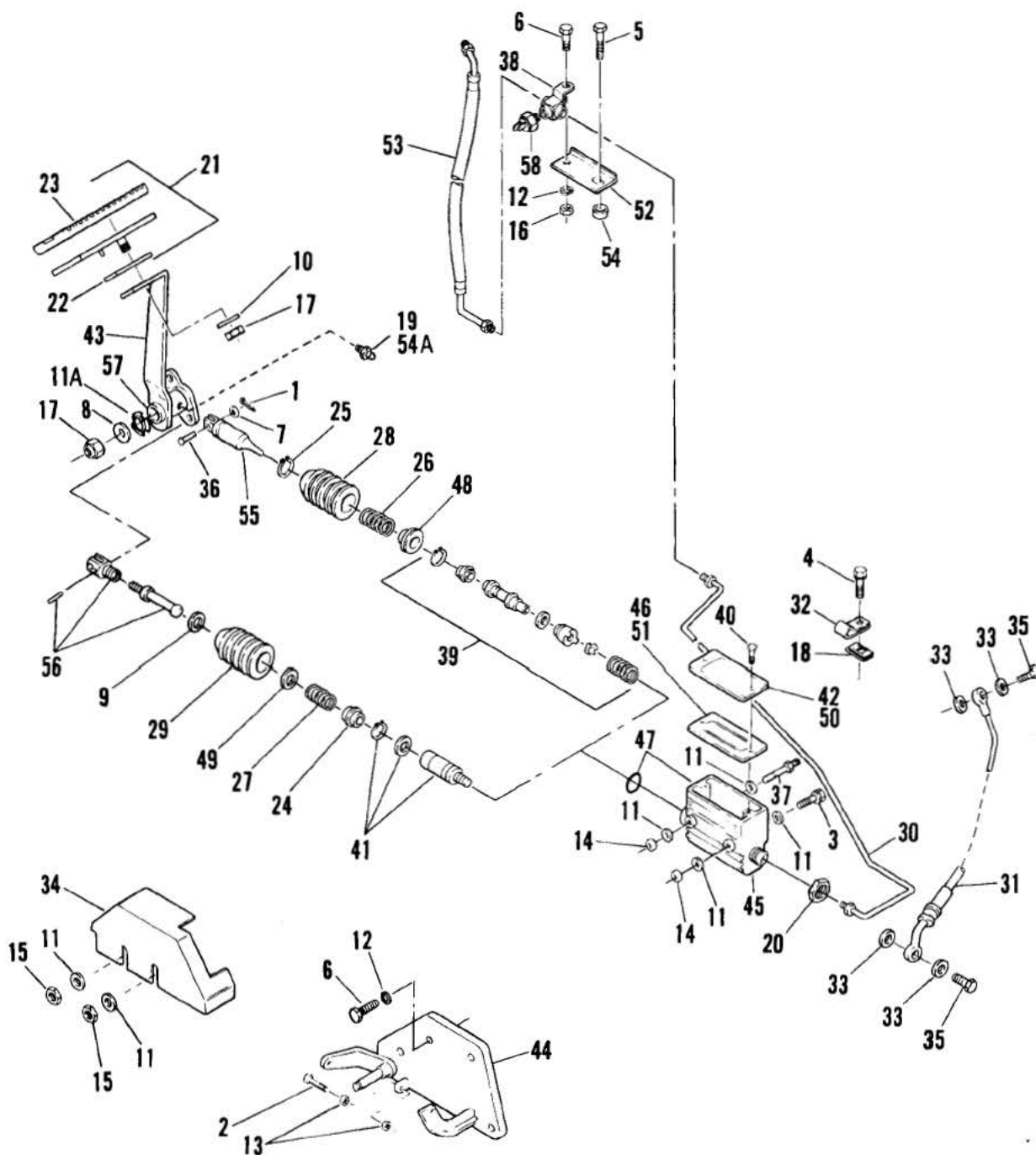
REAR BRAKE CONTROL — FLST
