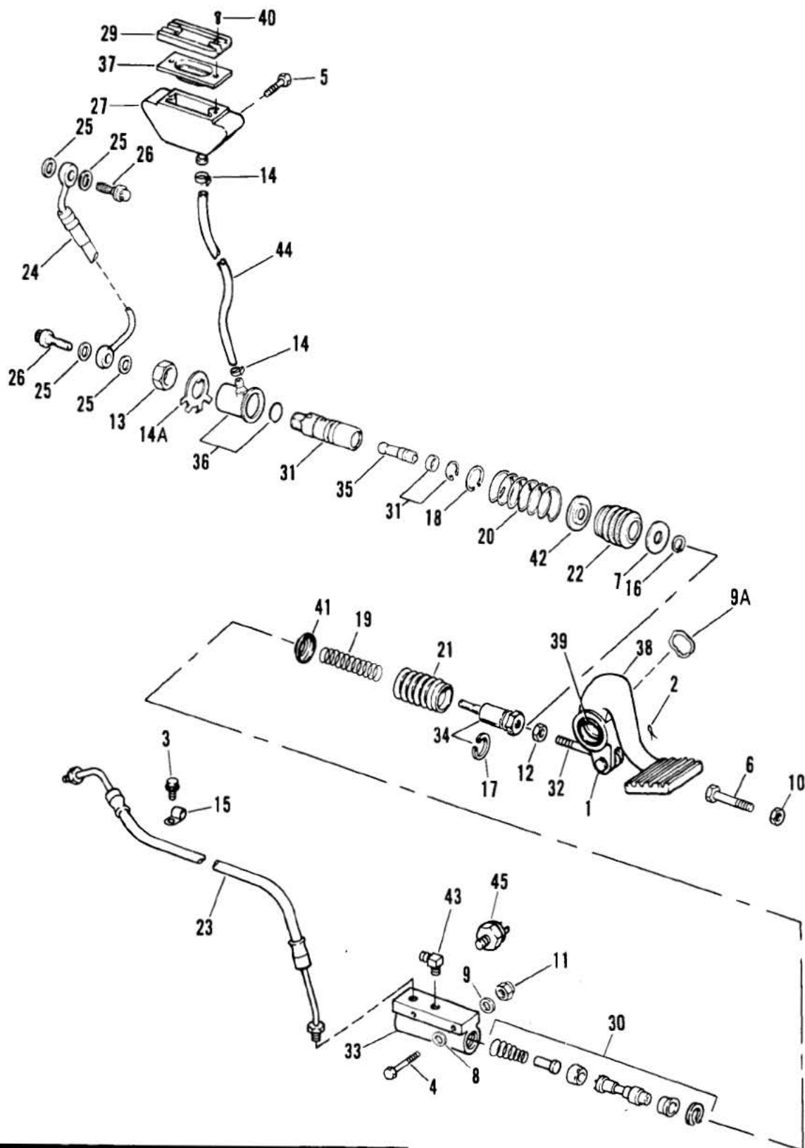
REAR BRAKE CONTROL — FXR
