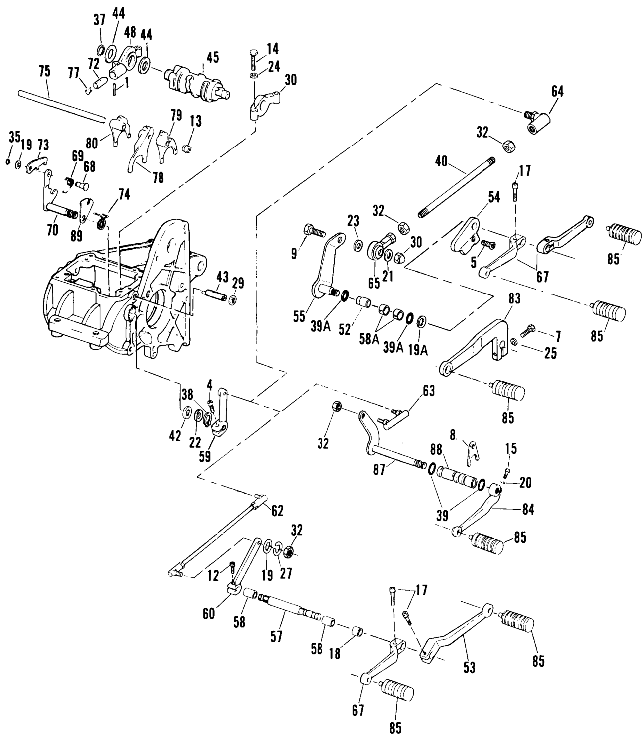
GEAR SHIFTER
