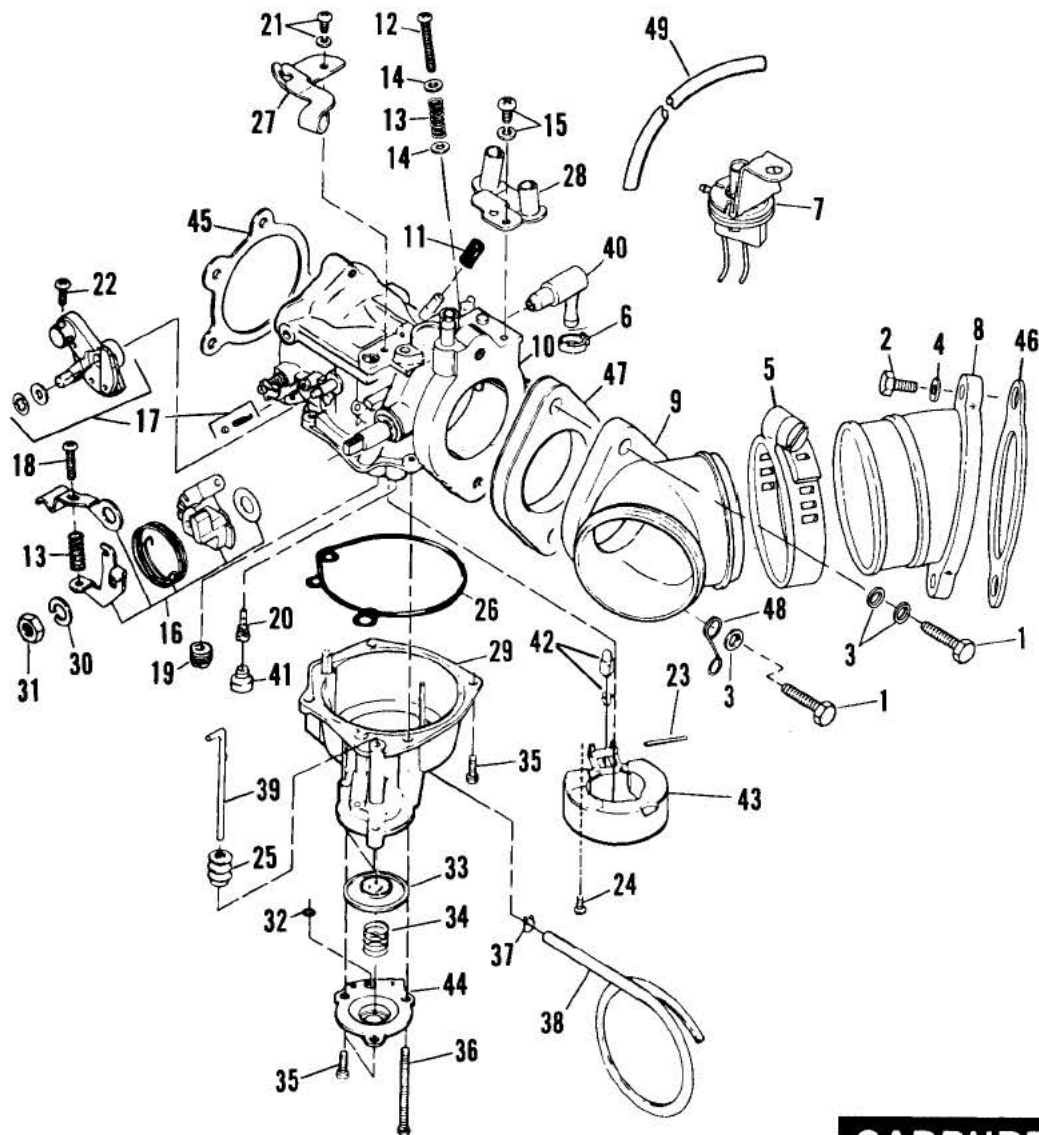
CARBURETOR 1987 TO 1989
