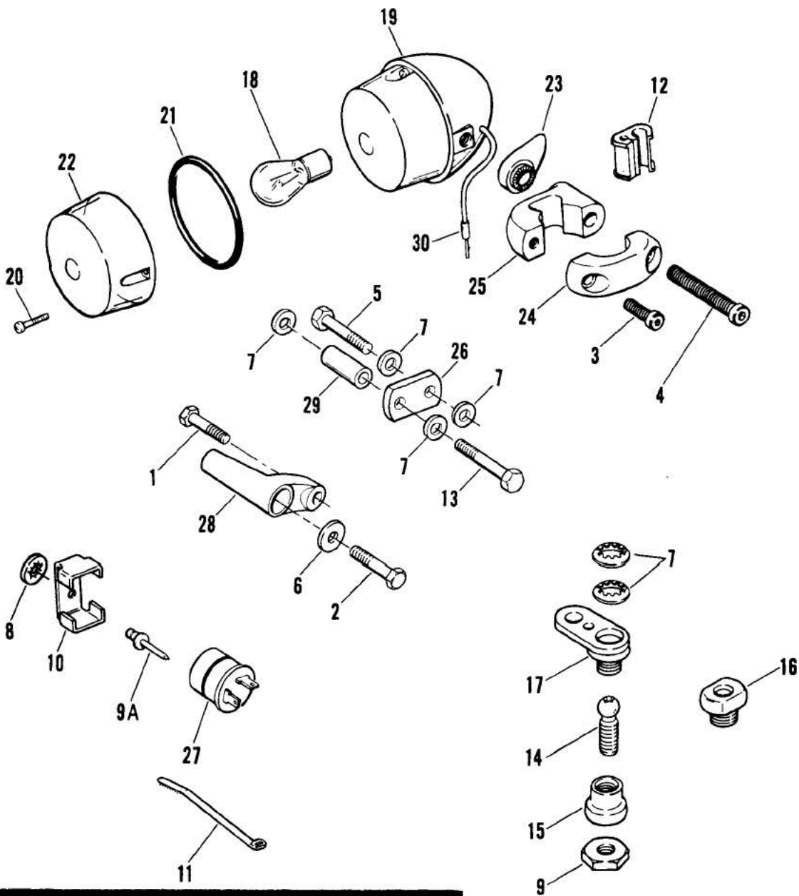
FRONT TURN SIGNALS — FXR, FXRS, FXLR & SOFTAIL
