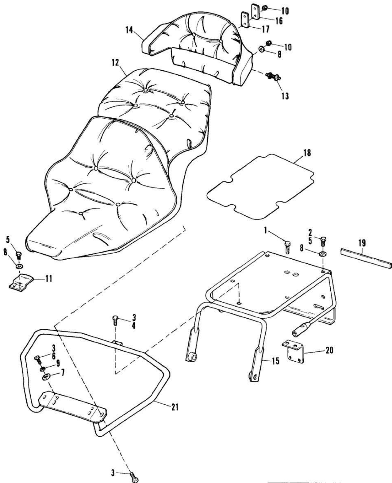
SEAT & LUGGAGE RACK — FLT
