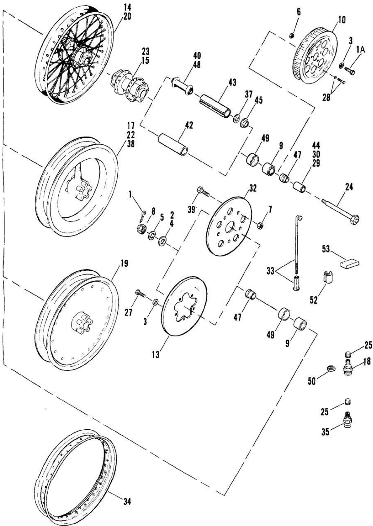
REAR WHEEL
