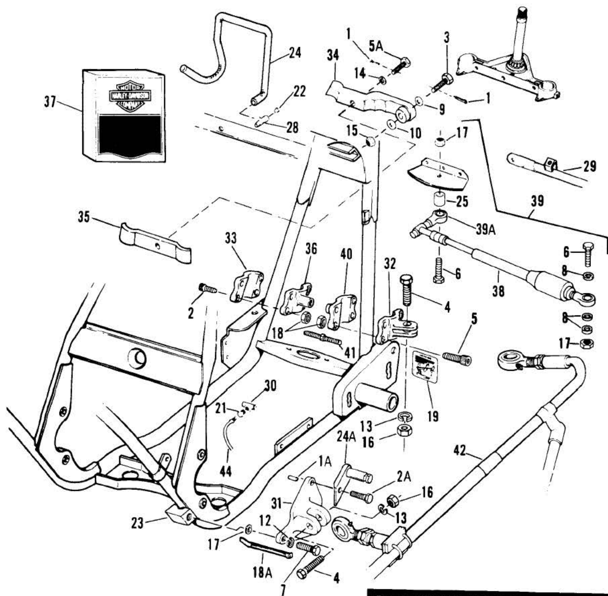
SIDECAR CONNECTION KIT — TLE
